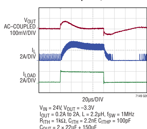
Transient Response, DCM
